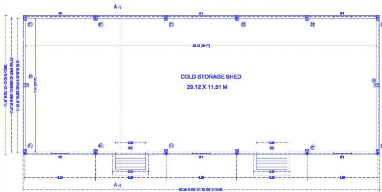
COLD STORAGE SHED PLAN
