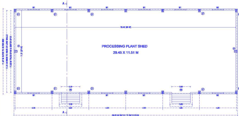
PROCESSING PLANT SHED PLAN
