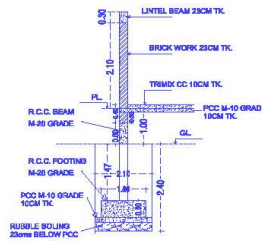
SECTION OF FOOTING
