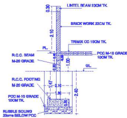
SECTION OF FOOTING
